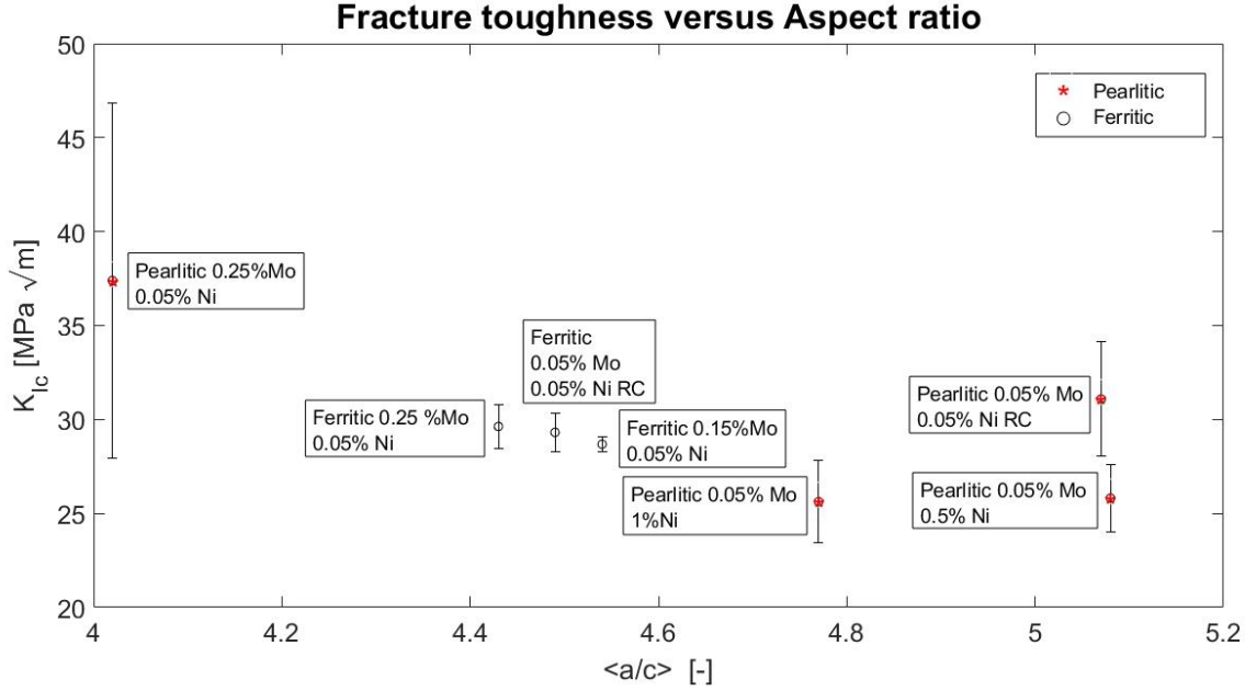
Figure 4.10: Relation between fracture toughness and graphite aspect ratio values for the specimens tested.
