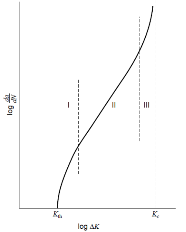
Figure 2.7: Crack growth stages [26].
