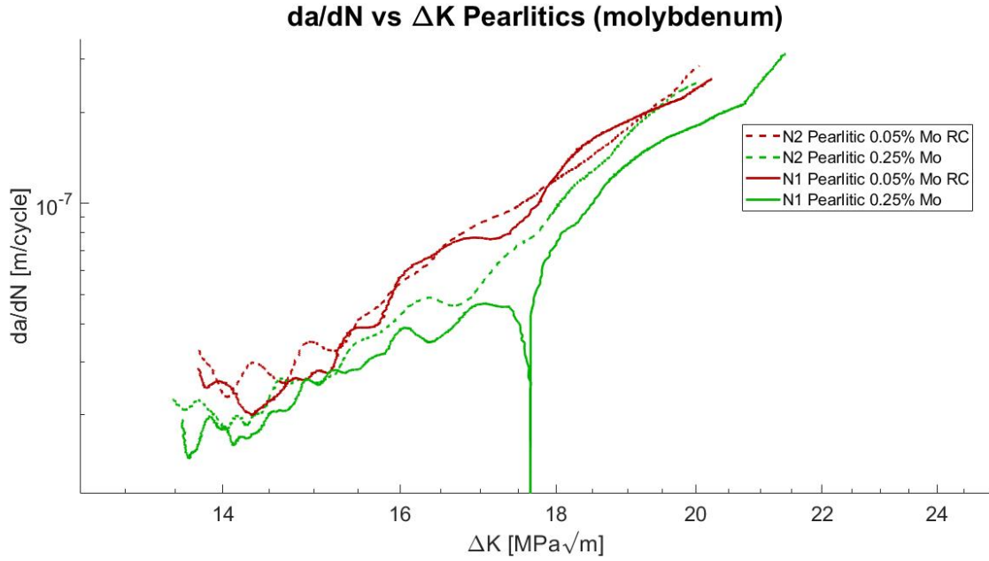
Figure 4.3: Fatigue crack growth rate versus the stress intensity factor range for the pearlitic specimens with molybdenum and reference composition, including tests N°1 and N°2.
