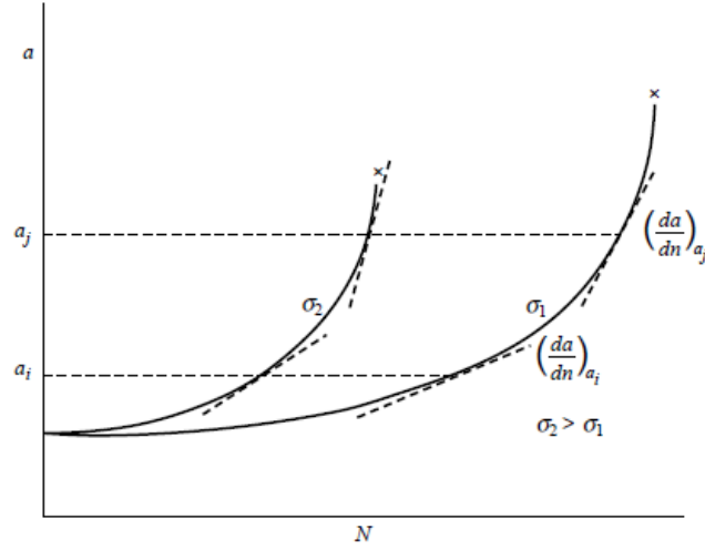
Figure 2.8: Stress effect on the fatigue crack growth rate from Deformation and fracture mechanics of engineering chapter 10 [26]
