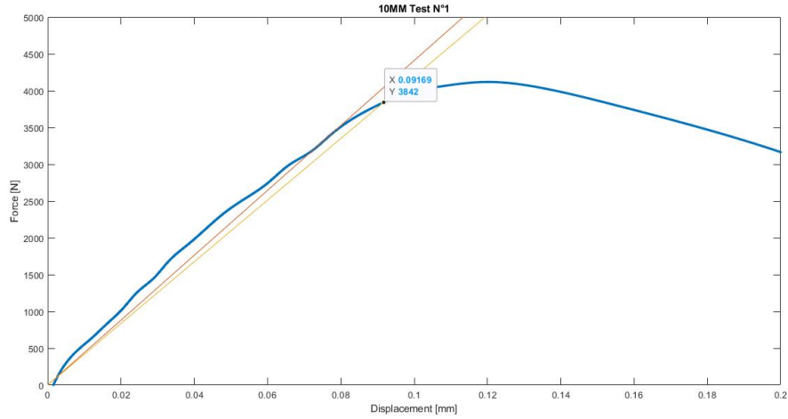
Figure 3.6: Chart of load [N] vs displacement [mm] for the specimen 10MM Pearlitic 0.5% nickel.
