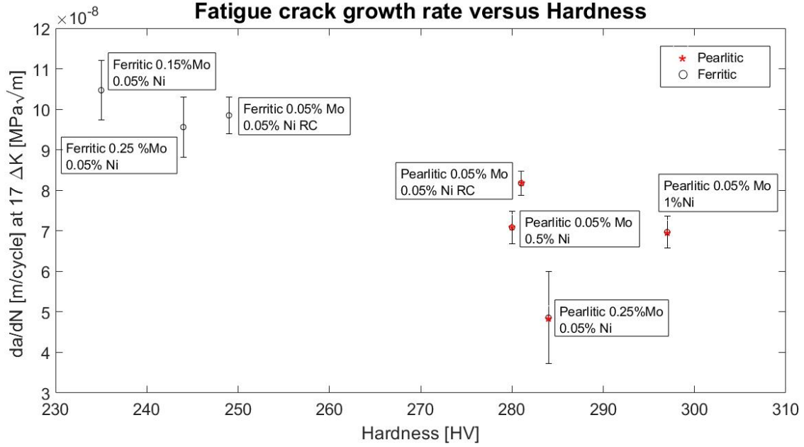
Figure 4.8: Fatigue crack growth rate at 17 \text{ MPa}\sqrt{m} versus hardness of all specimen tested.
