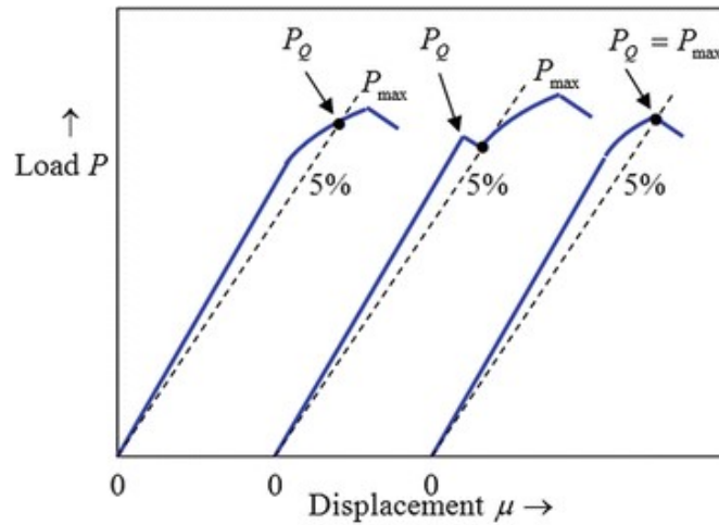
Figure 3.7: Types of load vs displacement curves.
