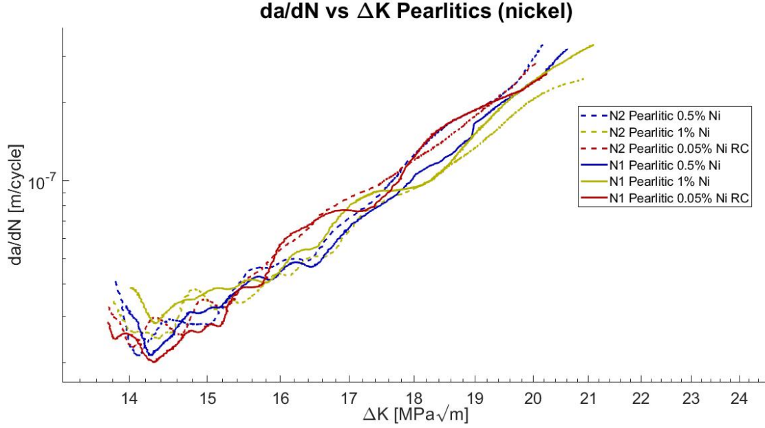
Figure 4.4: Fatigue crack growth rate versus the stress intensity factor range for specimens with nickel and reference composition. Tests N°1 and N°2 included.
