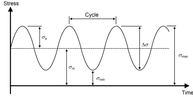
Figure 2.4: Description of cyclic parameters [22].
