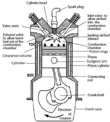
(a) Illustration of a mobile engine parts, including the cylinder head.
