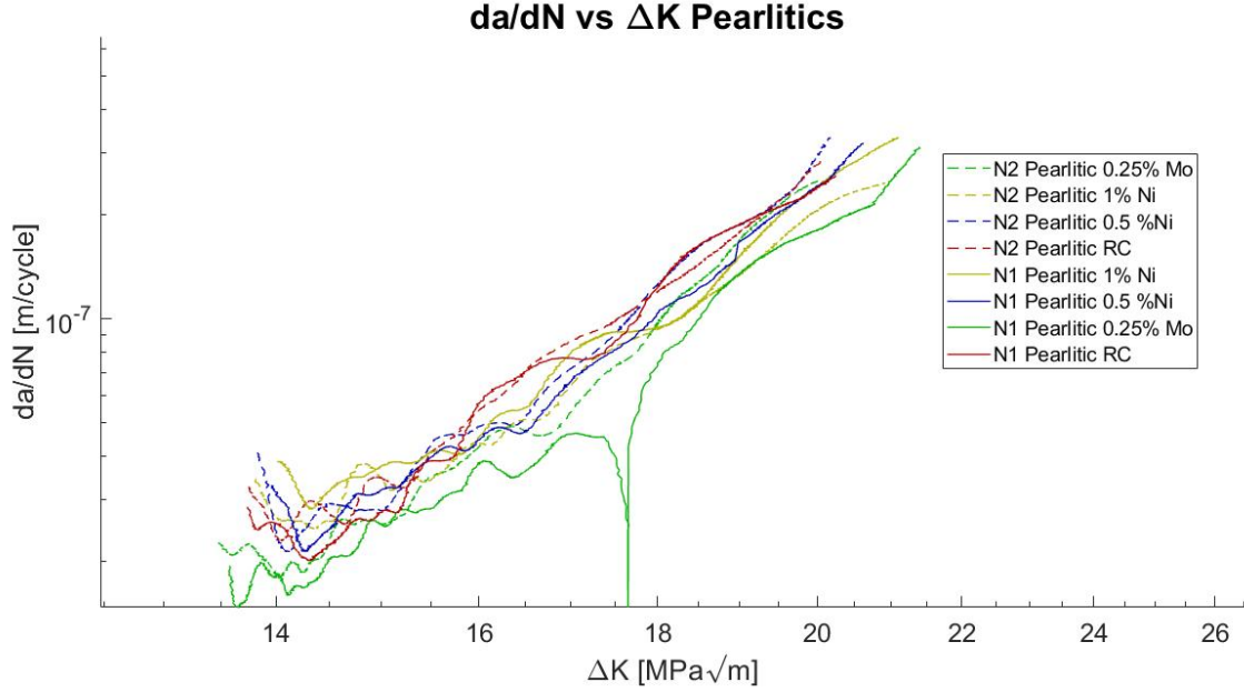
Figure 4.5: Fatigue crack growth rate versus the stress intensity factor range for pearlitic specimens. Includes tests N°1 and N°2.
