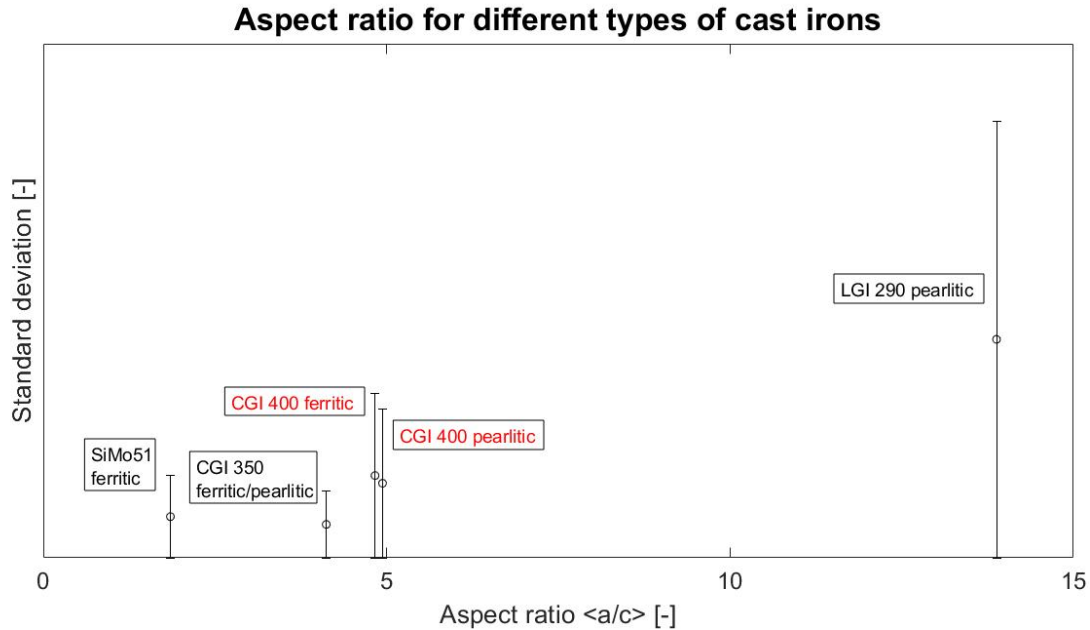
Figure 4.6: Chart of aspect ratio for lamellar (LGI290), compacted (CGI400, CGI350) and nodular iron (SiMo51) tested in the research paper "On the correlation between microstructural parameters and the thermo-mechanical fatigue performance of cast iron" [11].
