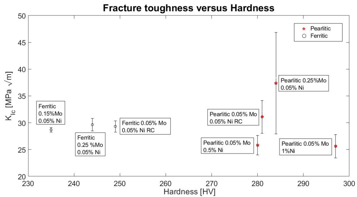
Figure 4.11: Relation between the fracture toughness and hardness values for the specimens tested.
