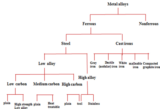
Figure 2.1: Classification of Metal Alloys from Concepts in Physical Metallurgy. [16]
