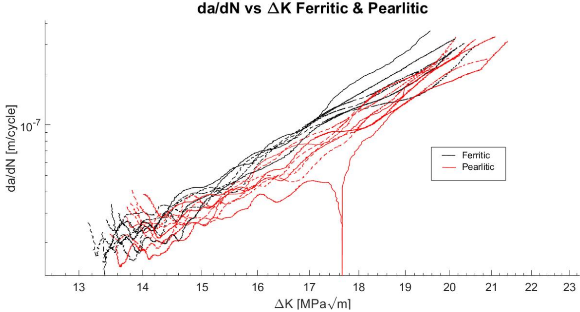
Figure 4.1: Fatigue crack growth rate versus the stress intensity factor range for the pearlitic and ferritic specimens, tests N°1 and N°2.
