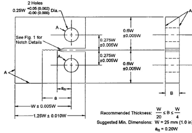
Figure 3.2: Specimen configuration (C(T)), for the fatigue crack growth rate test.
