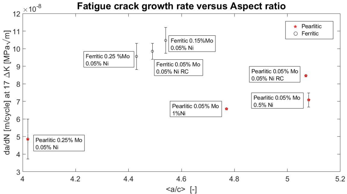
Figure 4.7: Fatigue crack growth rate at 17 \text{ MPa}\sqrt{m} versus aspect ratio for all specimen tested.
