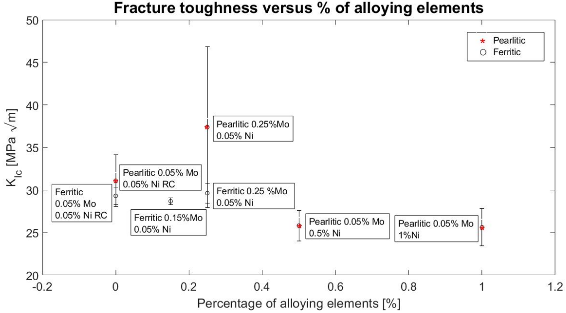
Figure 4.9: Relation between the fracture toughness values and the amount of alloying elements for the compositions tested.
