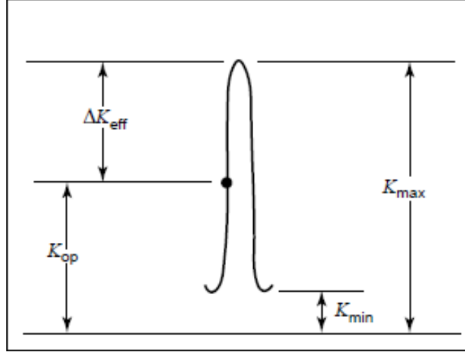
Figure 2.6: Stresses involve in crack surface opening [26].
