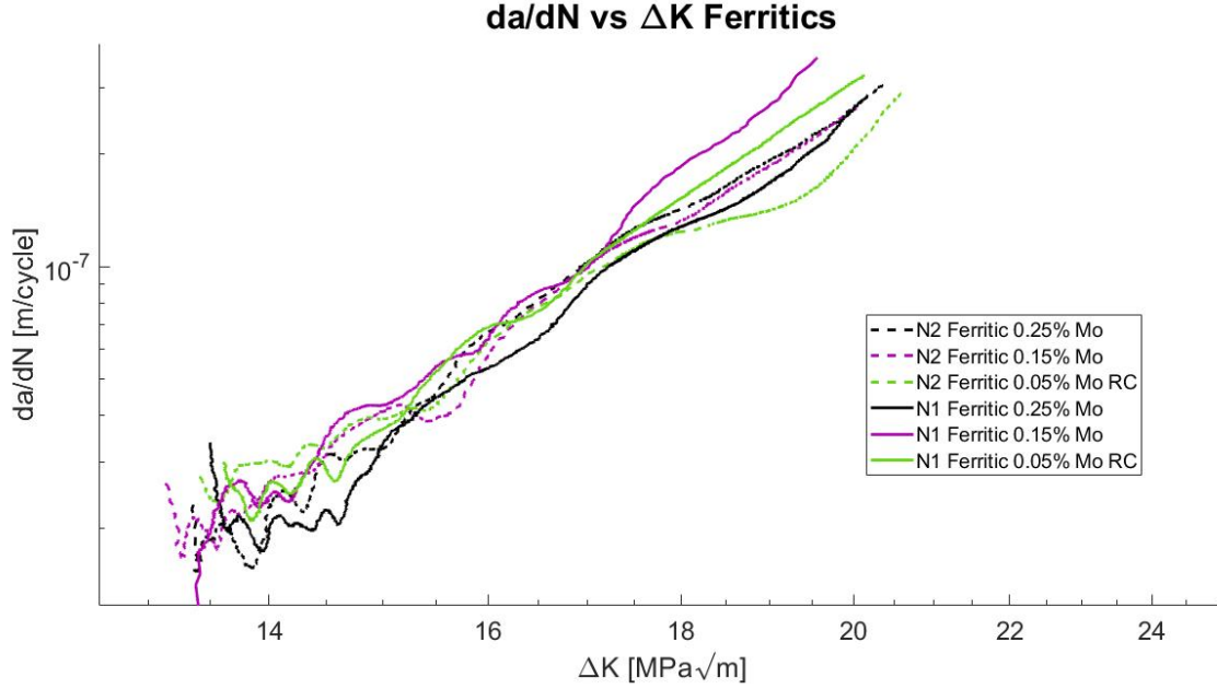
Figure 4.2: Fatigue crack growth rate versus the stress intensity factor range for the ferritic specimens, tests N°1 and N°2 included.
