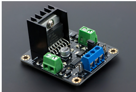
Figura 5.3: MD1.3 2A Dual Motor Controller SKU DRI0002
