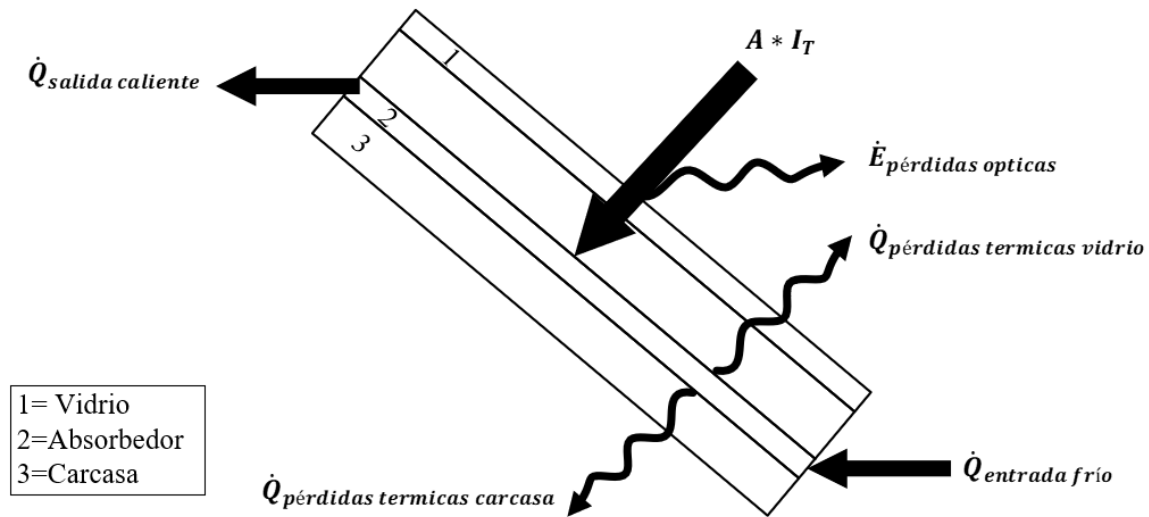
Figura 6.8: Balance energa colector plano (Fuente: Adaptacin Solar District Heating Guidelines)
