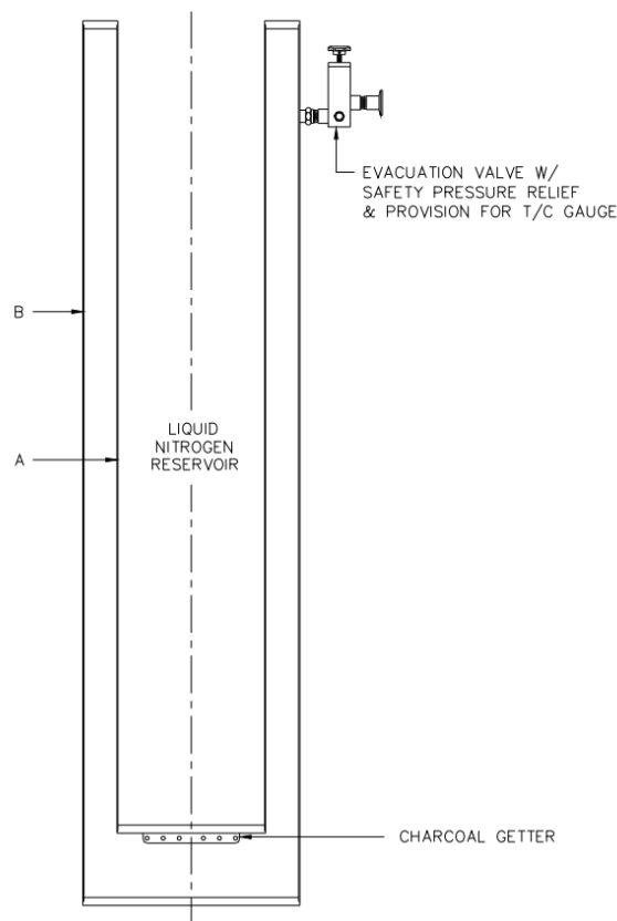
FIGURE 2.1 OPEN NECK LIQUID NITROGEN DEWAR
