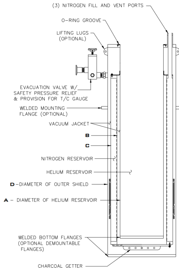
FIGURE 2.2 OPEN NECK NITROGEN SHIELD LIQUID HELIUM DEWAR
