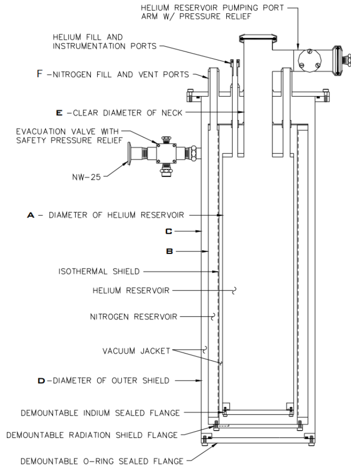
FIGURE 2.6 DETACHABLE TAIL LIQUID HELIUM DEWAR
