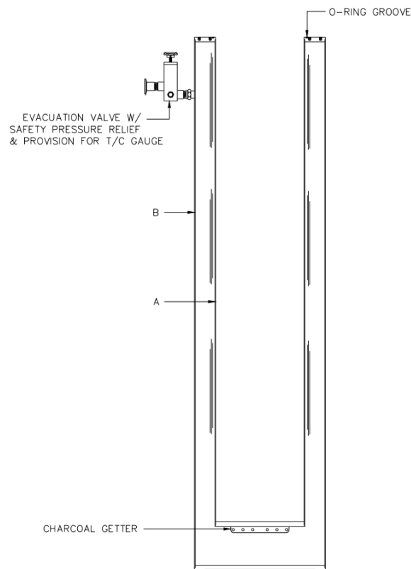
FIGURE 2.3 OPEN NECK SUPERINSULATED LIQUID HELIUM DEWAR
