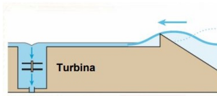
Figura 17: Rebalse [25]
