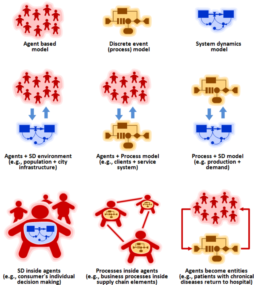
Figura 3.4. Representación de las arquitecturas de modelado multiparadigma. (Borshchev, The big book of simulation modeling: multimethod modeling with AnyLogic 6., 2013)
