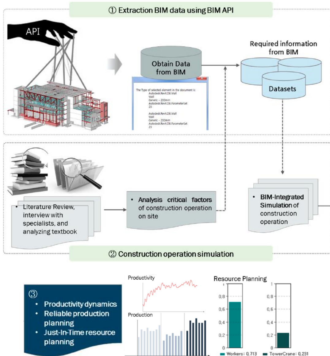
Figura 3.5. Marco de simulación BIM. (WoonSeong, Soowon, JeongWook, & June-Seon, 2016)
