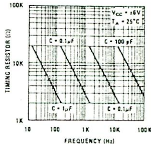
VCO Frequency
