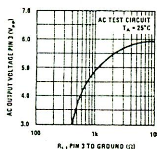
Square Wave Output Characteristics
