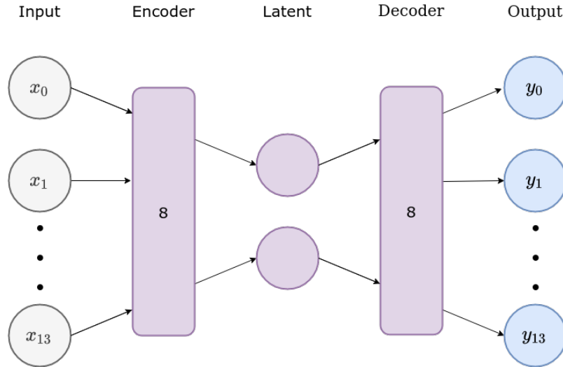
Figure 19: Autoencoder architecture.
