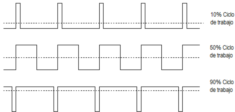
Figura 3.2: Control PWM.
