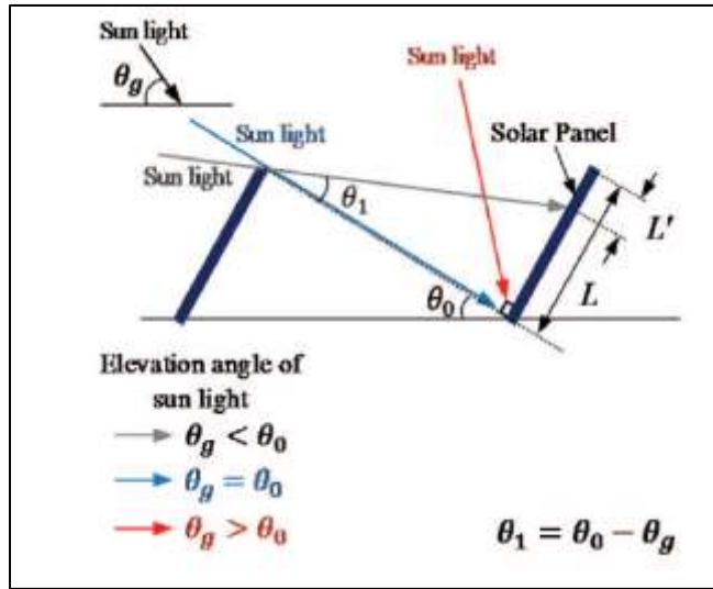
Figura 2.6 Caso (a), panel PV sin reflector [7].
