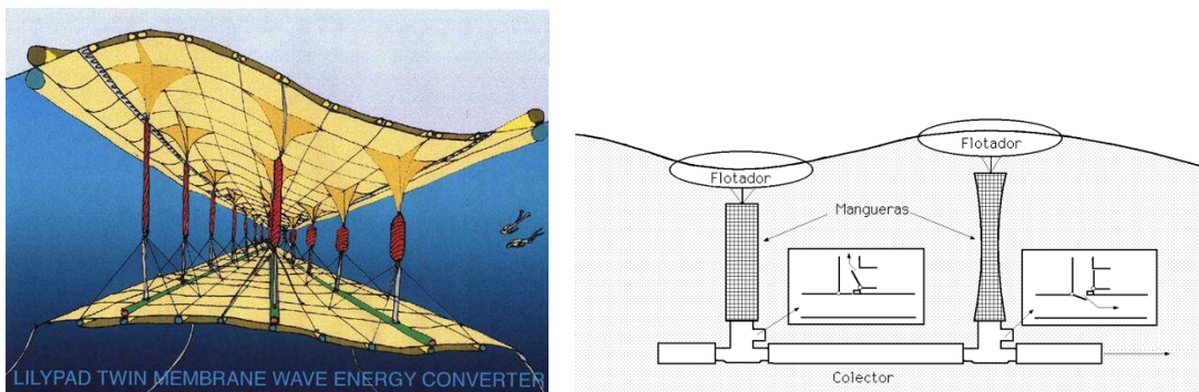
Figura 3.8 Lilyppad
